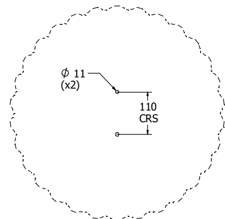
Required Host Panel Fixing Detail
