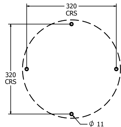
Required Host Panel Detail
