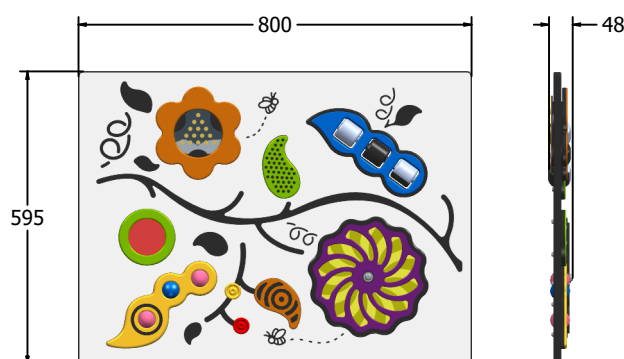
FISENP6 FISENP6-AL-WP Standard Panel Panel with Alu Posts
