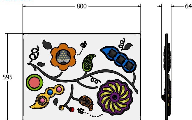
FISENP6 FISENP6-AL FISENP6-AL-WP Standard Panel Panel with Edge Slots for Alu Posts Panel with Alu Posts
