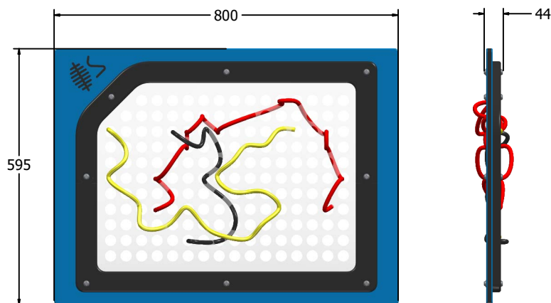
FIWEAVE6 Standard Panel FIWEAVE6-AL-WP Panel with Alu Posts
