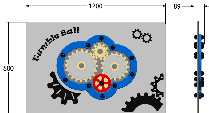
FITUMBLE3NGP Standard Panel FITUMBLE3NGP-AL-WP Panel with Alu Posts
