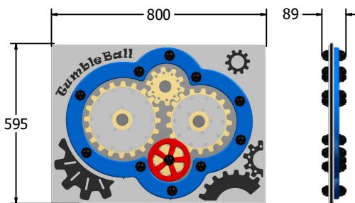
FITUMBLE6NGP Standard Panel FITUMBLE6NGP-AL-WP Panel with Alu Posts
