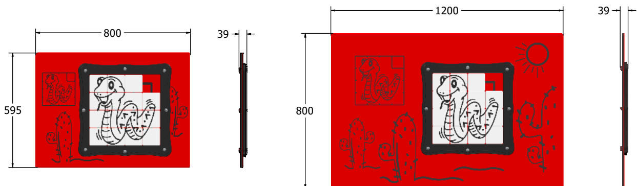
FITSSNAKE3 Standard Panel FITSSNAKE3-AL-WP Panel with Alu Posts
