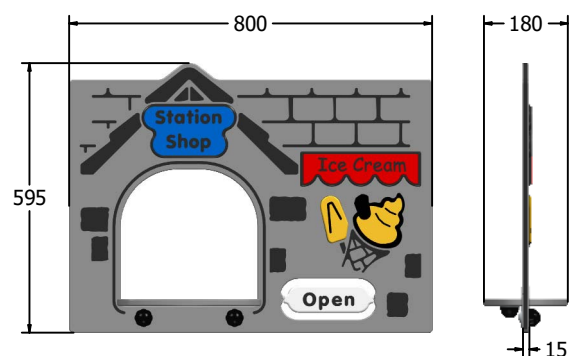
FISTAT6 Standard Panel FISTAT6-AL-WP Panel with Alu Posts
