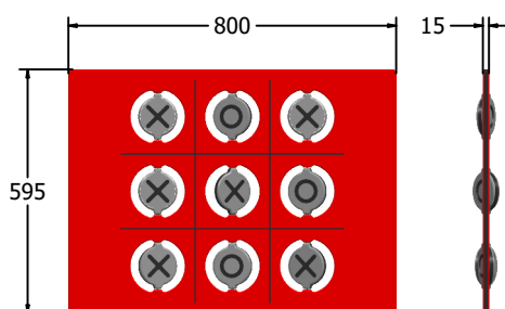
FISPNOUGHTS6 FISPNOUGHTS6-AL-WP Standard Panel Panel with Alu Posts
