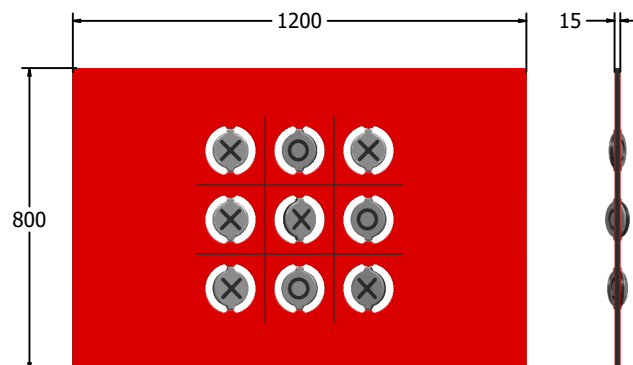
FISPNOUGHTS3 FISPNOUGHTS3-AL-WP Standard Panel Panel with Alu Posts
