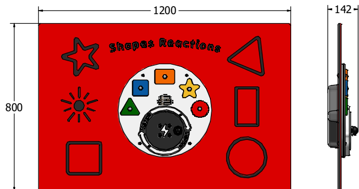
FIPTSHREACTRG3 Standard Panel FIPTSHREACTRG3-AL-WP Panel with Alu Posts
