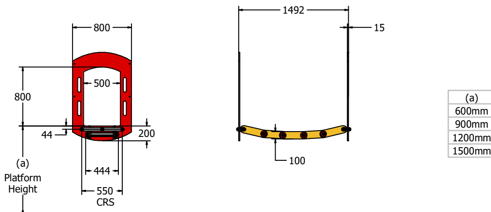
Slip Resistant Ladder Rung
