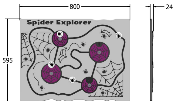
FIEXSPIDER6 FIEXSPIDER6 -AL-WP Standard Panel Panel with Alu Posts
