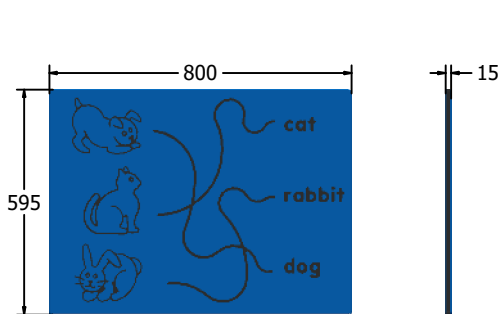
FIDOGTR6 Standard Panel FIDOGTR6-AL-WP Panel with Alu Posts
