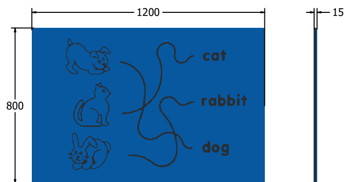
FIDOGTR3 Standard Panel FIDOGTR3-AL-WP Panel with Alu Posts
